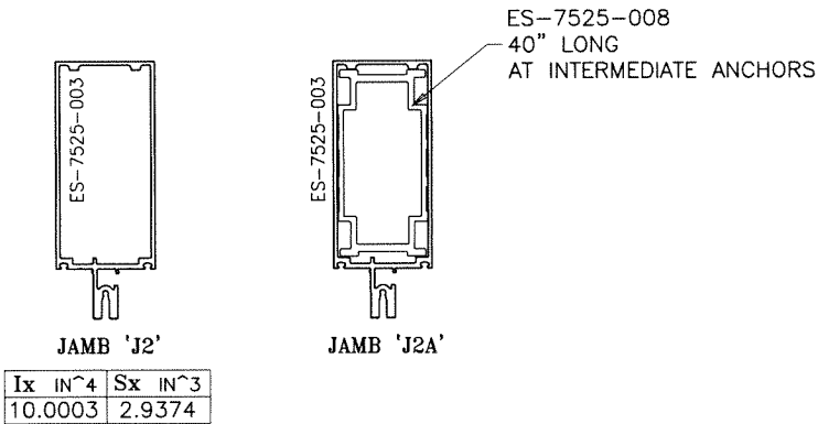
JAMBS TWIN SPAN TABLES
