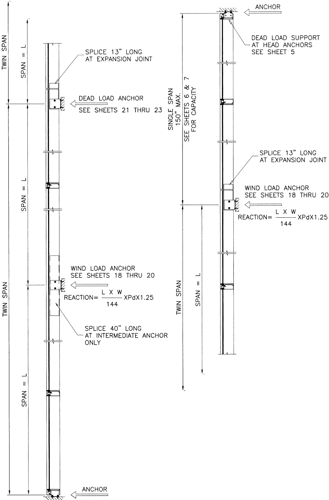
MULTIPLE SPANS
