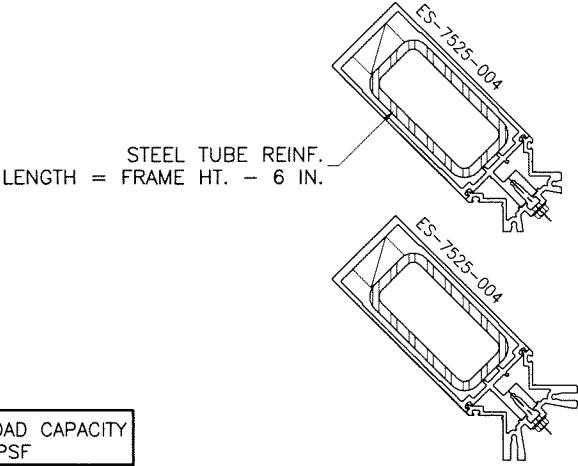
CORNER MULLION W/ STEEL REINF.
