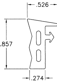
INT. GLAZING GASKET G8
