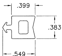
EXT. GLAZING GASKET G6 (LAMINATED GLASS)
