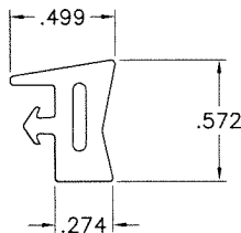
EXT. GLAZING GASKET G1 (INSUL. LAM. GLASS)
